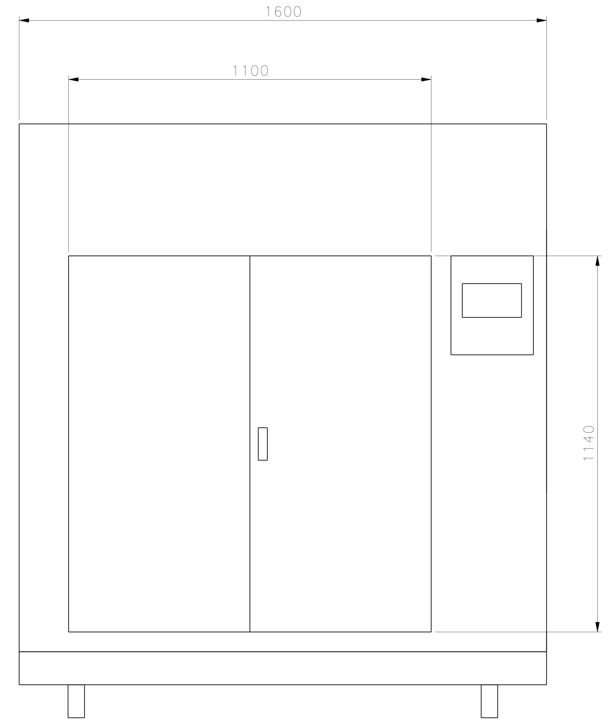
FRONT VIEW
