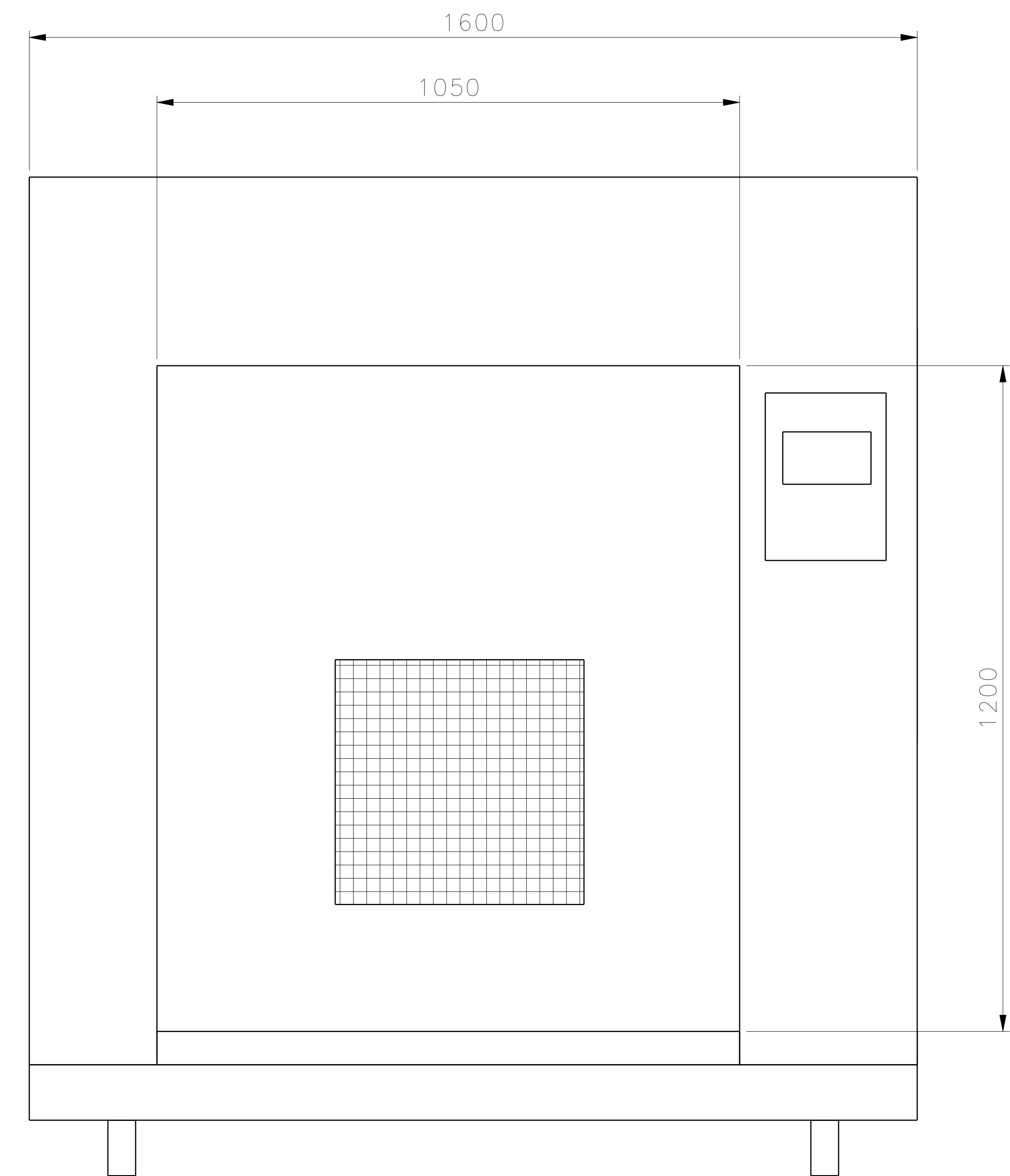
Auxiliary view A Scale: 1:6
