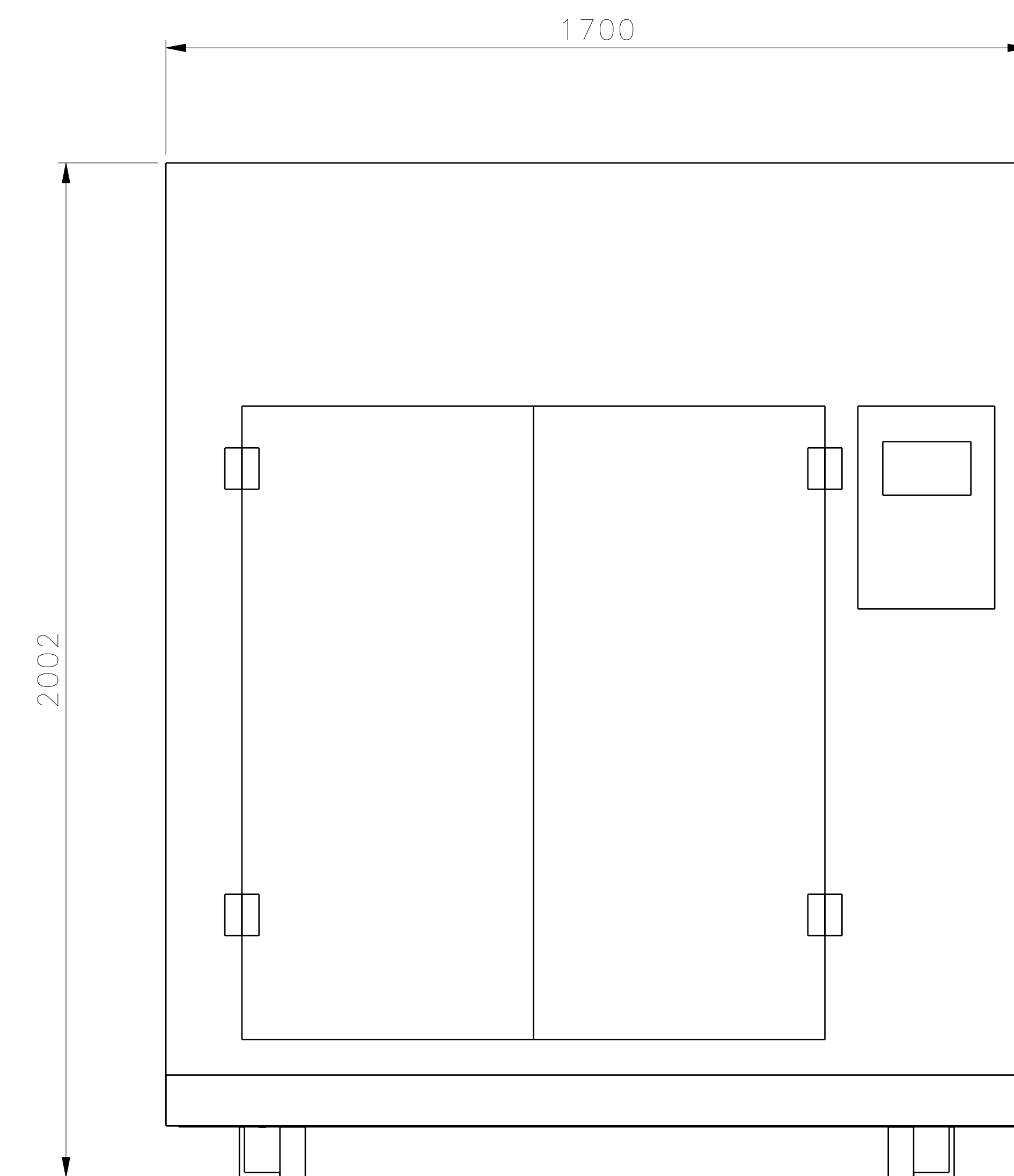
Front view Scale: 1:8
